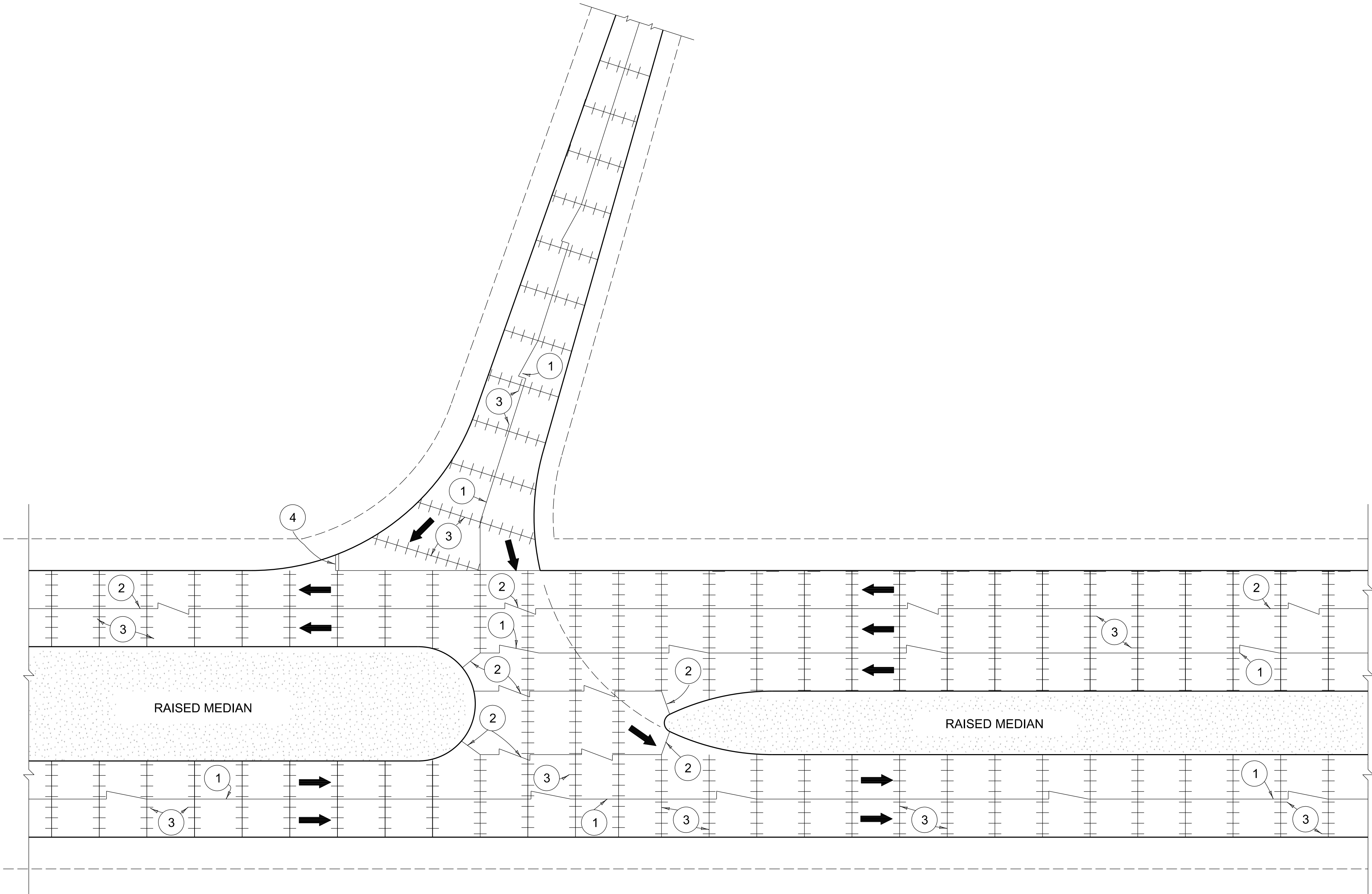
INTERCHANGE RAMP DETAIL ENTRANCE TO MINOR FOUR LANE ROAD
